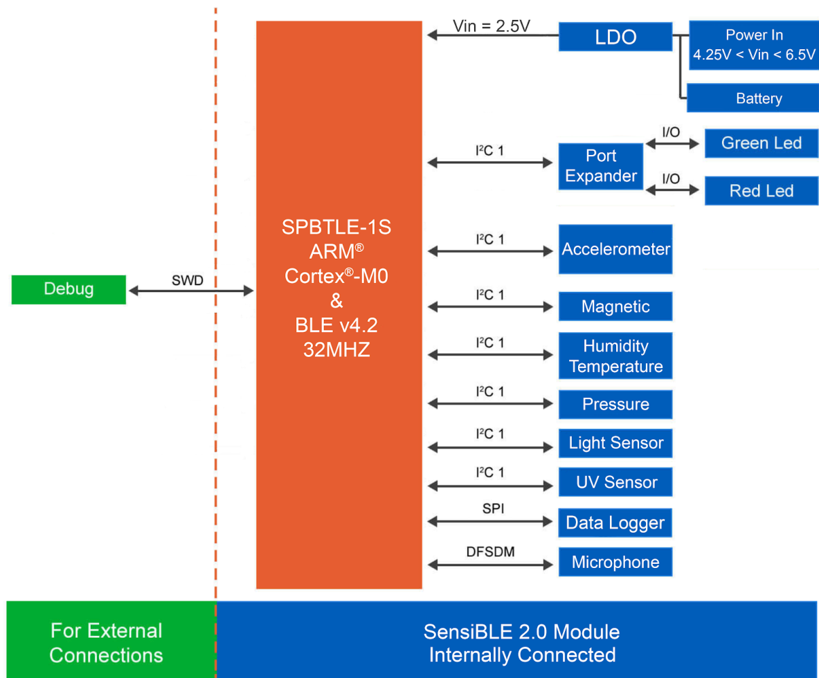
Figure 2 - SensiBLE 2.1 , Connections Diagram
