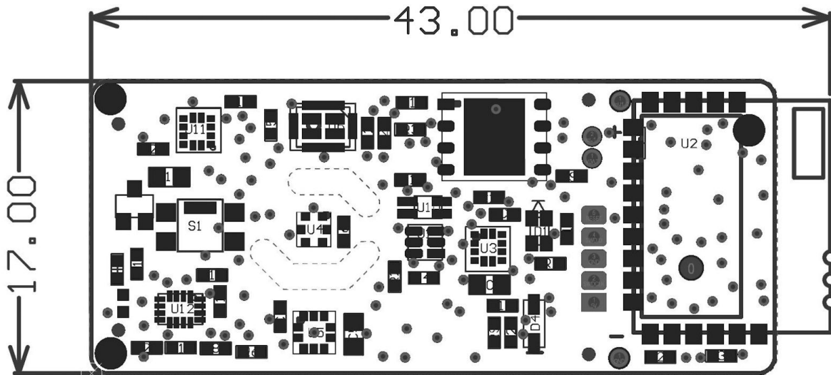
Figure 25 - SensiBLE 2.1 , Down View
