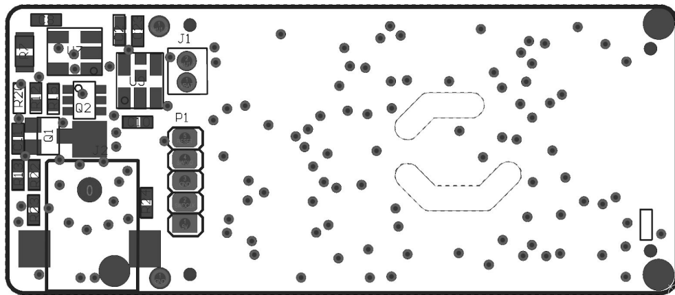
Figure 25 - SensiBLE 2.1 , Down View
